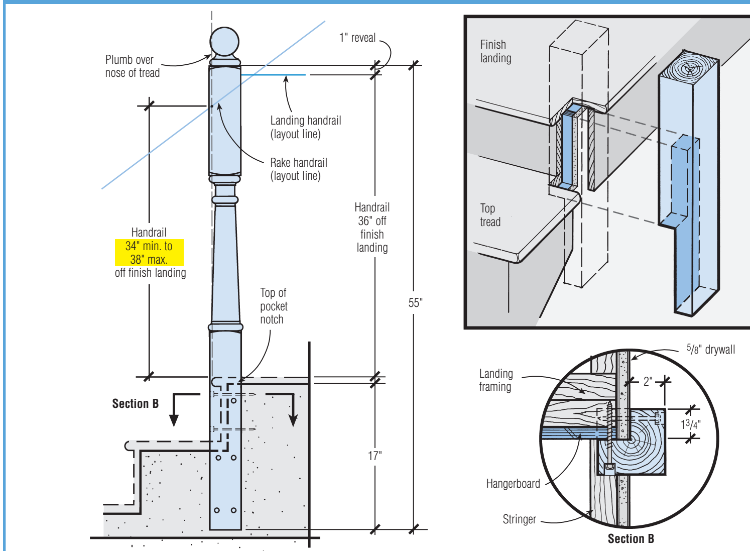
Figure 8-114. Landing Newel
