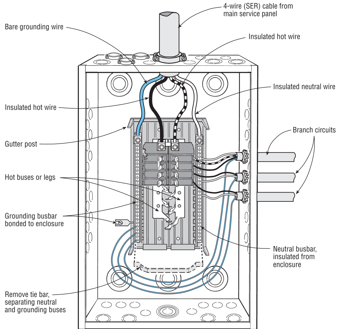
Figure 5-23. Termination of Grounds and Neutrals in Subpanel
