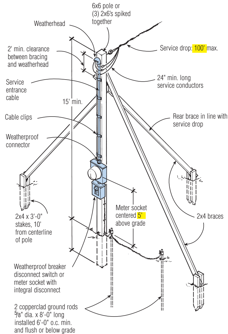
Figure 5-18. Typical Temporary Service
